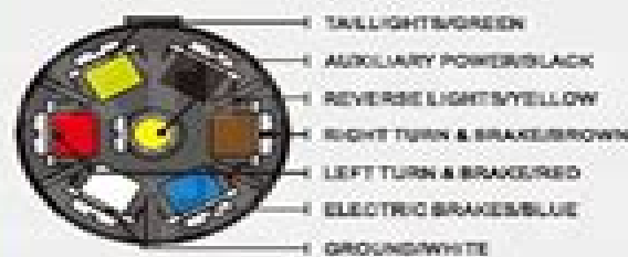
7 BLADE (RV STANDARD)
