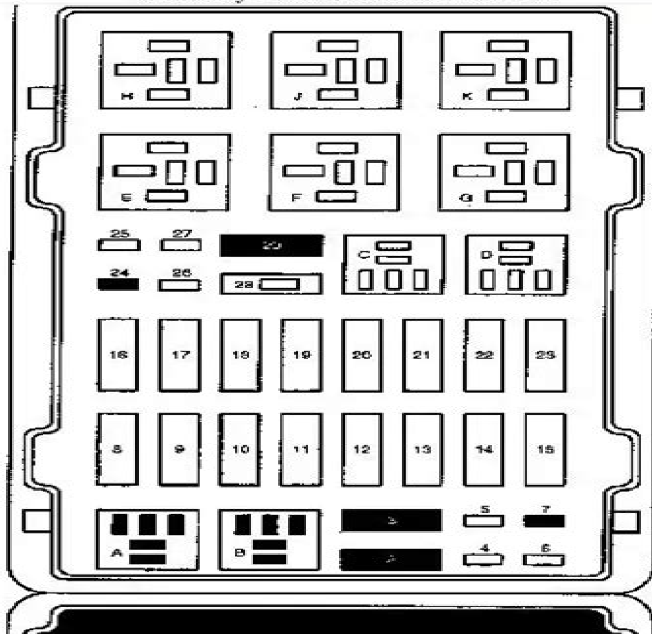
Fig. 7: Identifying Battery Junction Box Components
