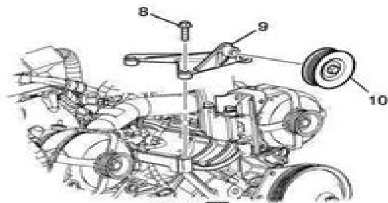
VIEW A (C42)
