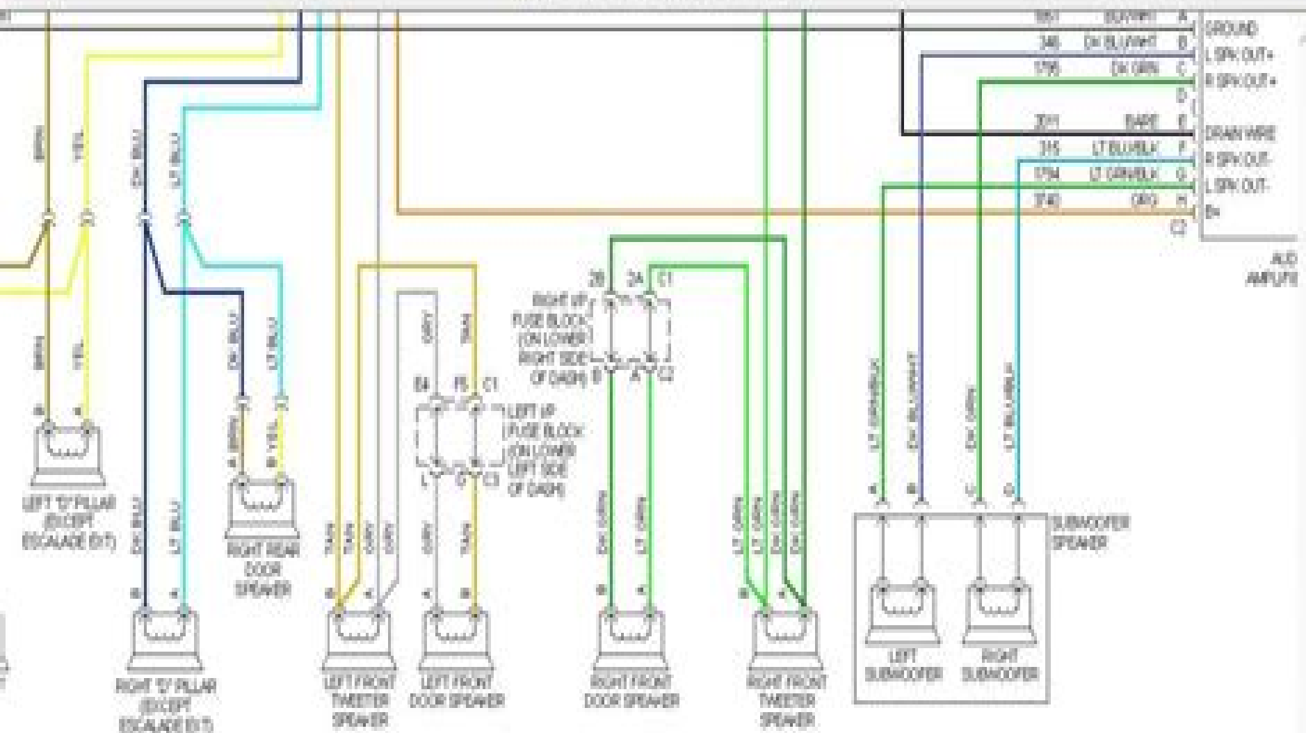
Fig. 14 Multi-Line Radio Circuit, W/ Rear Seat Audio (2 of 2)
