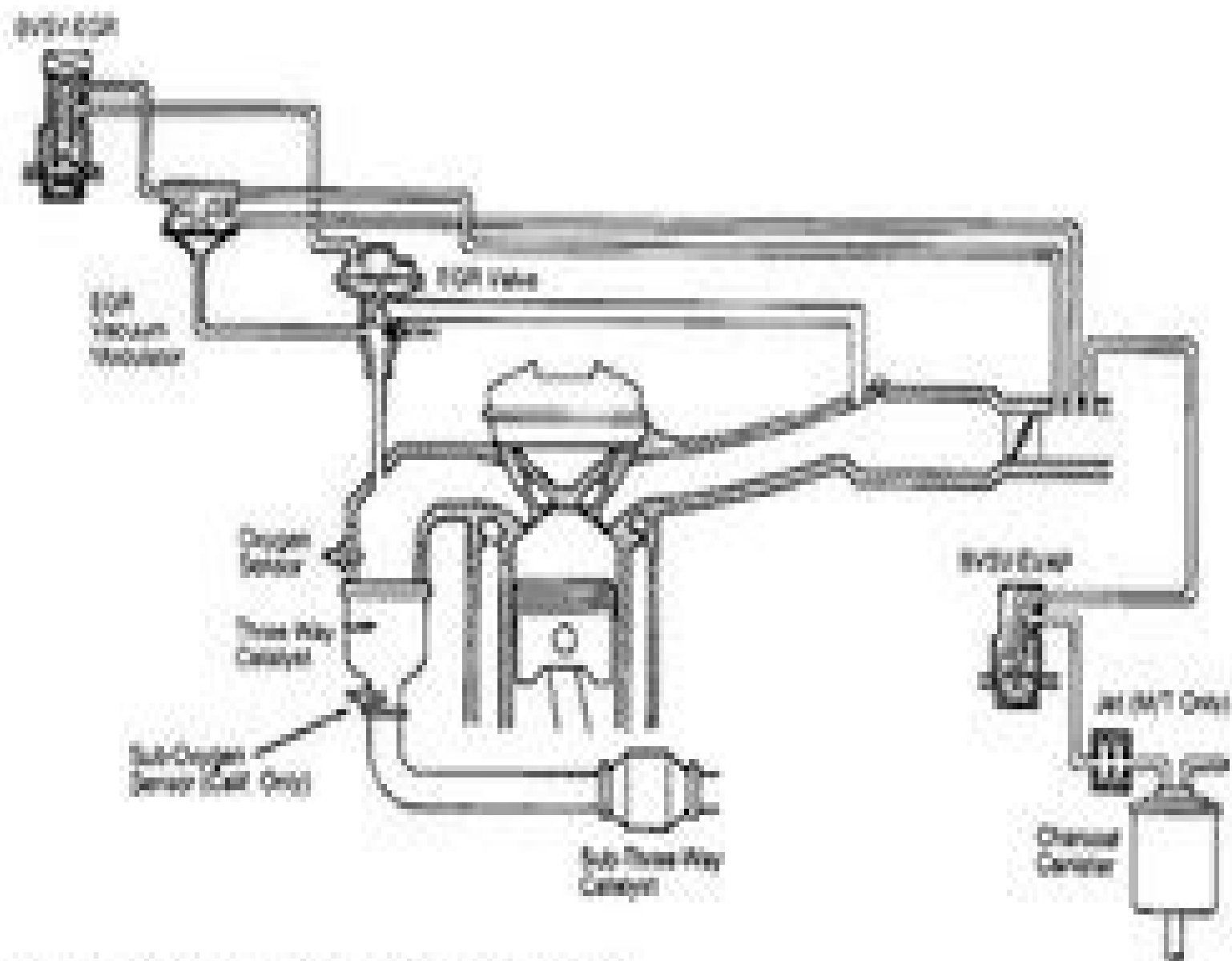
Fig. 2: Vacuum Diagram (Camry 2.0L 2 of 2) Courtesy of Toyota Motor Sales, U.S.A., Inc.
