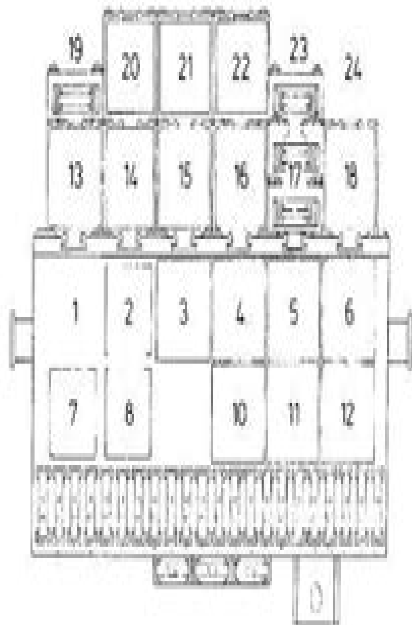
Relay locations
