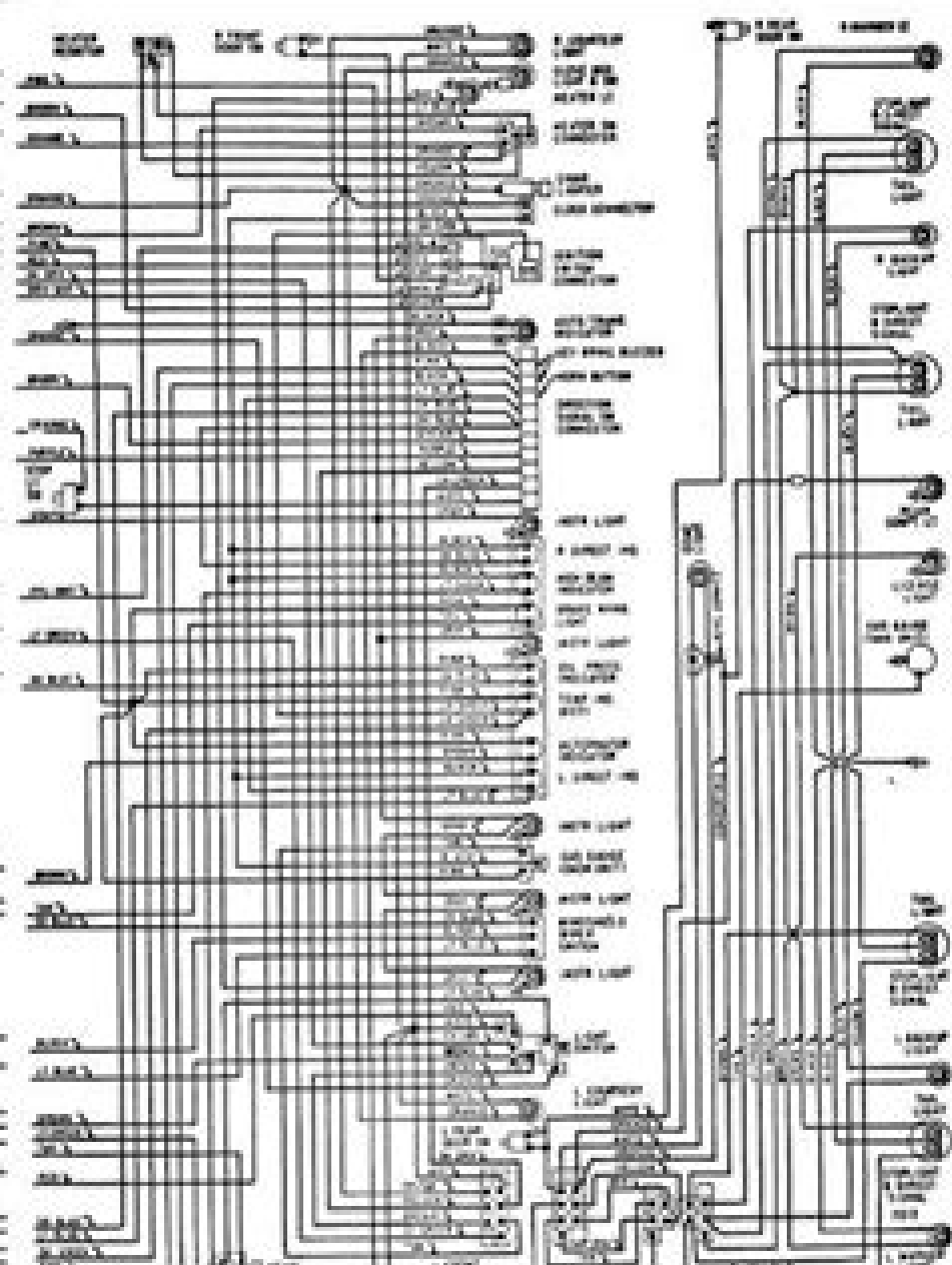
Fig 2: Wiring Diagrams - Chevrolet - Biscayne, Bel Air, Impala & Caprice
