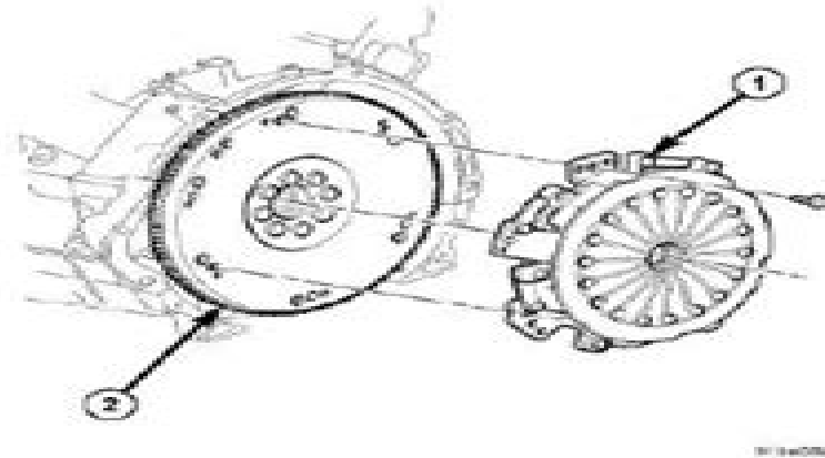
Fig. 15: Pressure Plate & Flywheel Courtesy of CHRYSLER GROUP, LLC
