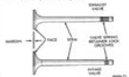
Fig. 81 Intake and Exhaust Valves
