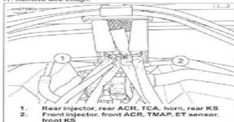
Figure 8-112. Breakout Harnesses
