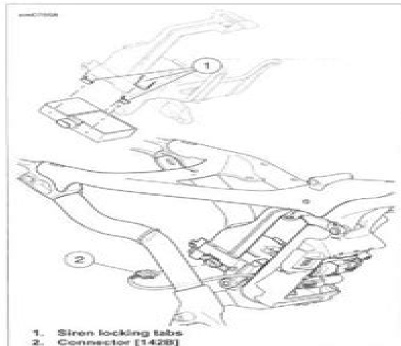
Figure 6-13. Smart Siren
