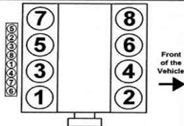
4.0L (VIN C) Engine Firing Order: 1-2-7-3-4-5-6-8 Distributorless ignition system
