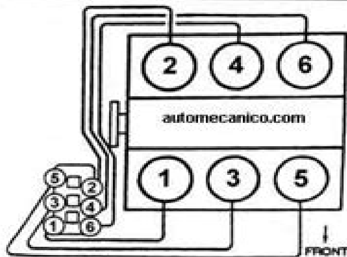
3.8L (VIN 1) Engine Firing Order: 1-6-5-4-3-2 Distributorless ignition system
