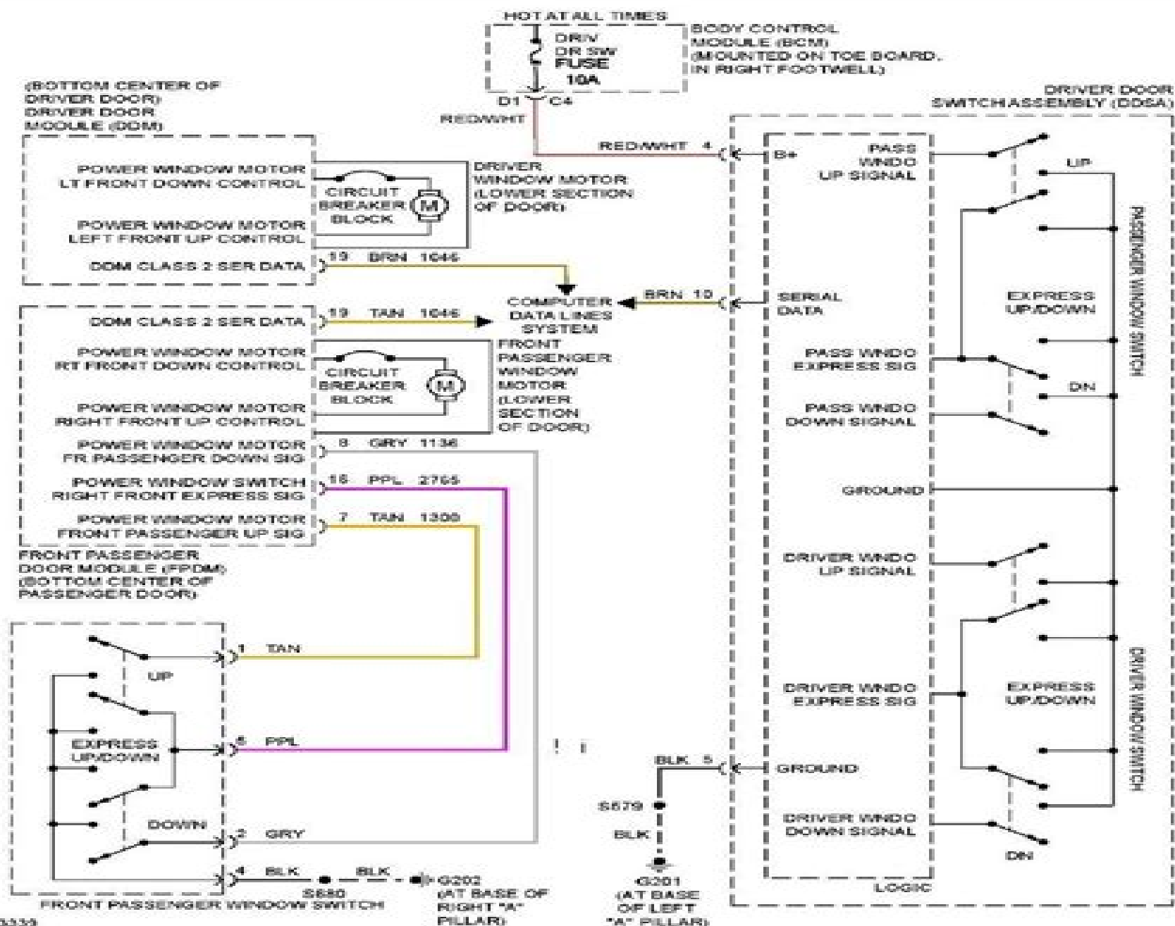
Fig. 63: Power Windows Circuit
