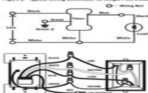
Figure 2 - Typical Wiring Schematic for Single Pole Installation
