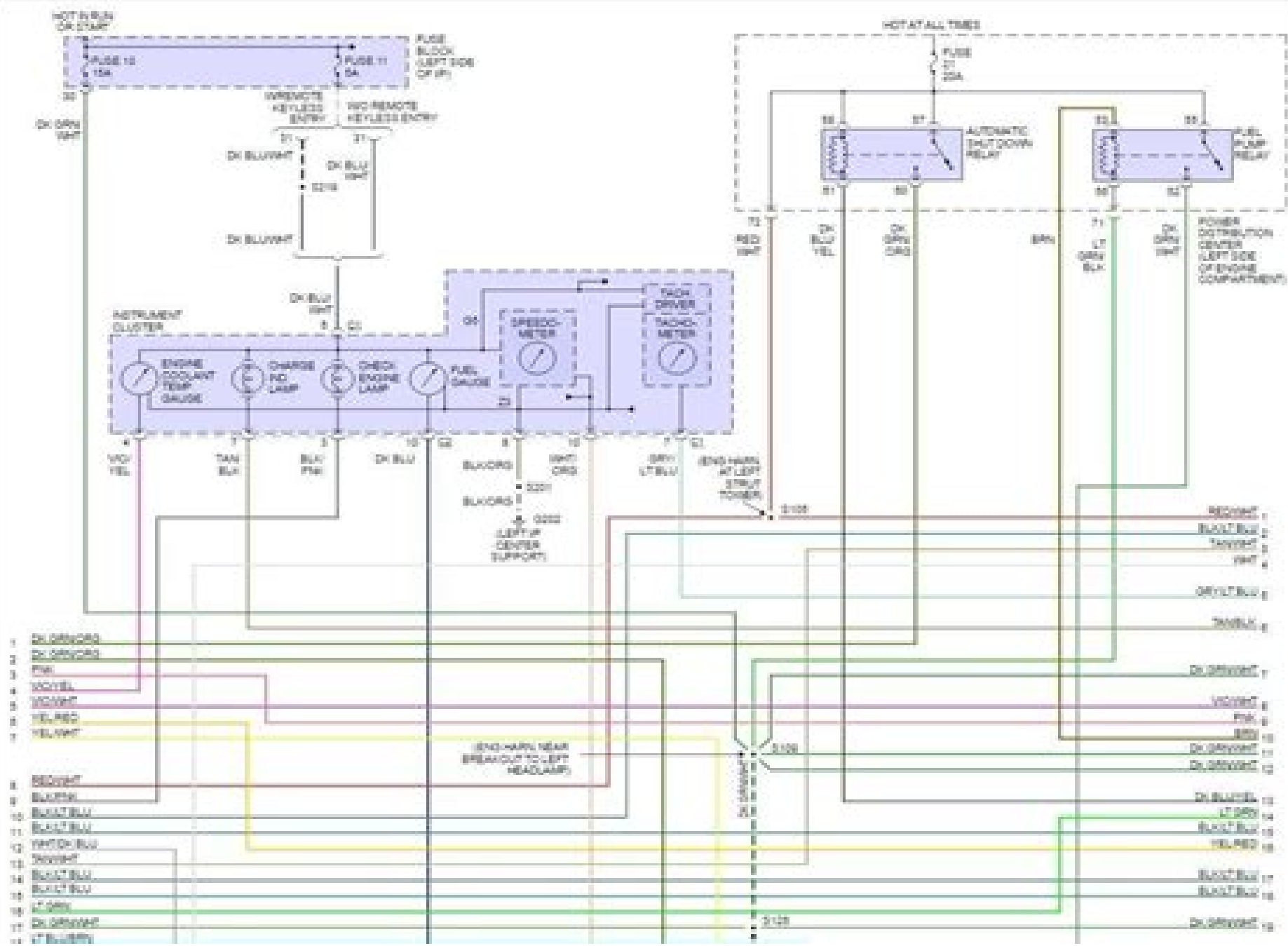
Fig 2: 2.0L Engine Performance Circuits (2 of 3)
