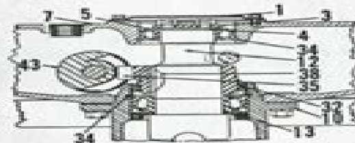
Fig. ACP—Models RC, and WC non-adjustable type axle version front support and main steering gear assembly.
