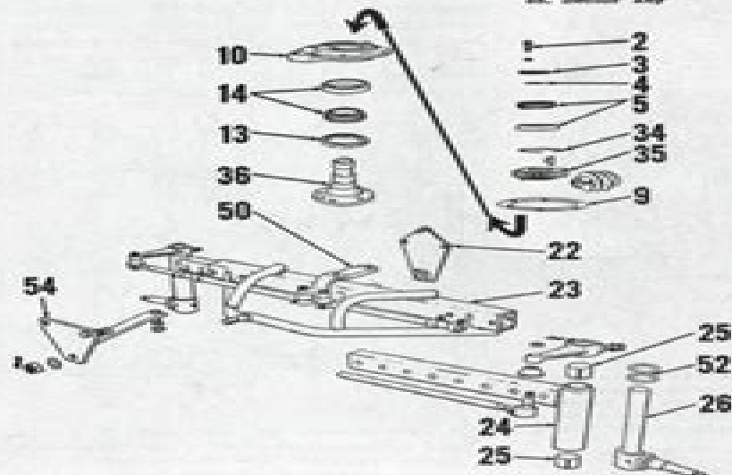
Fig. ACT—Models WD and WD-45 adjustable axle version main steering gear, and axle assembly.
