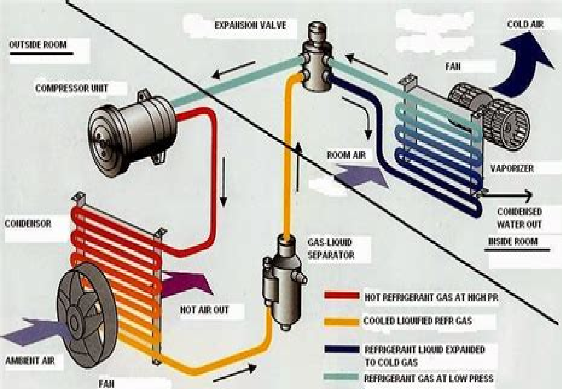
WORKING PRINCIPLE DIAGRAM OF AN AIR CONDITIONER UNIT
