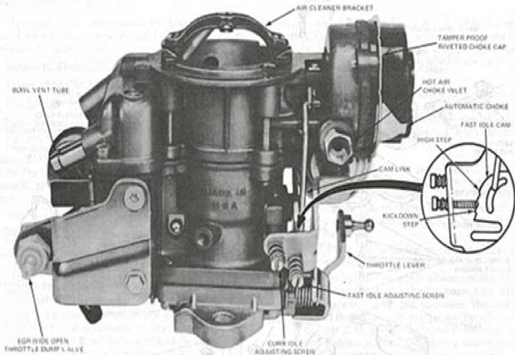
FIG. 1 YFA 1-V Carburetor—Rear View
