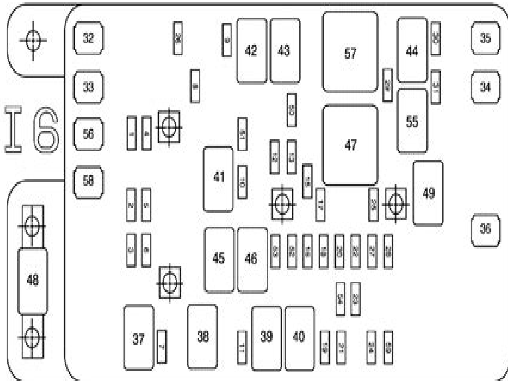
L6 Engine
