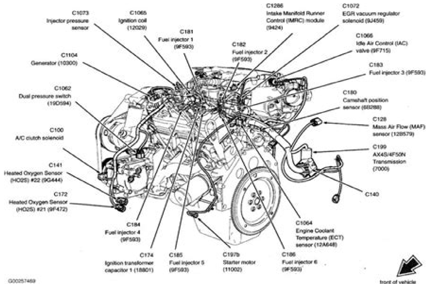
Fig. 1: Front Of Engine (2V)
