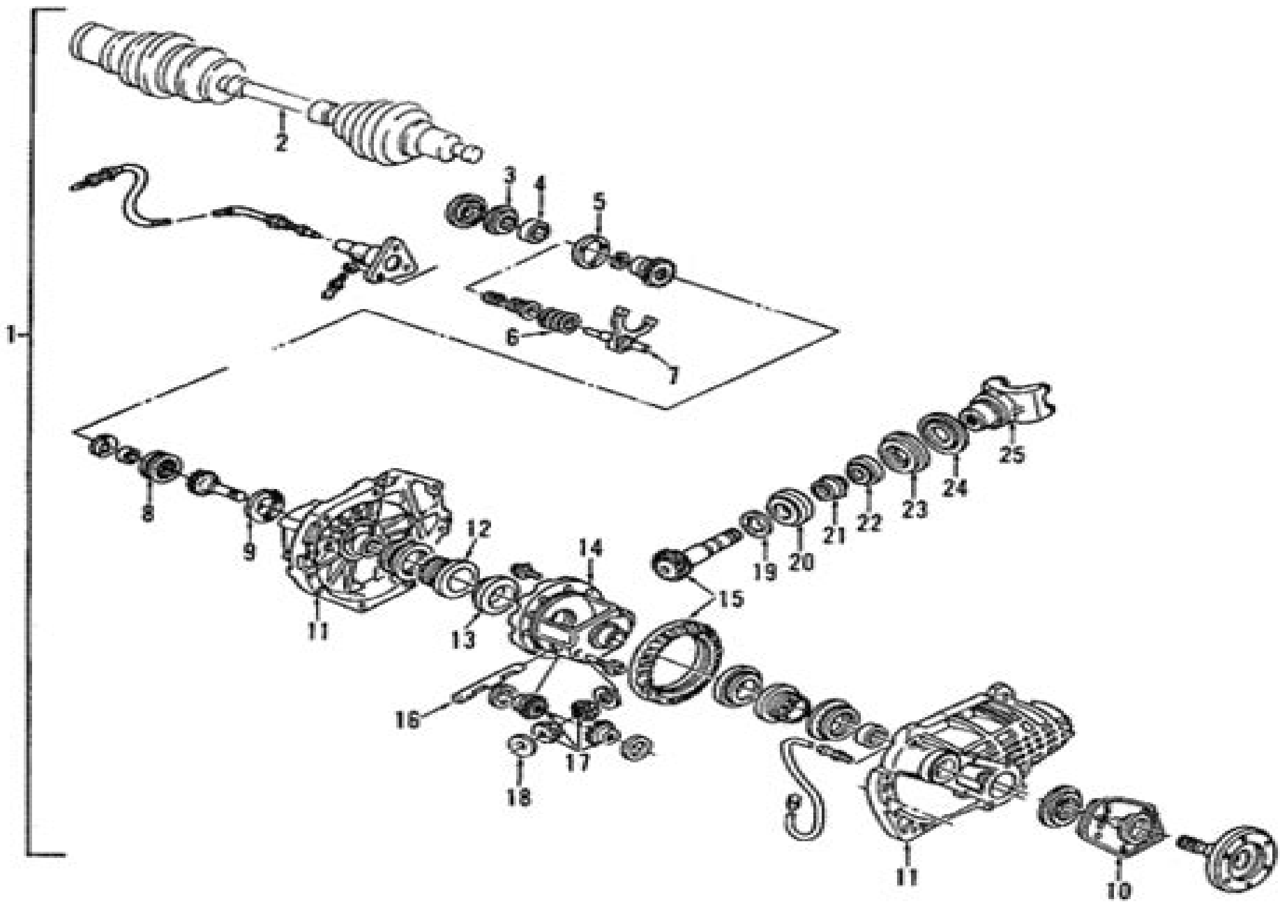
FRONT DRIVE AXLE - PART TIME 4WD
