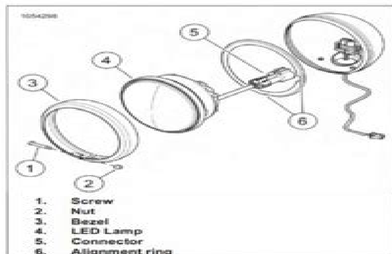
Figure 7-70. LED Auxiliary Lamp
