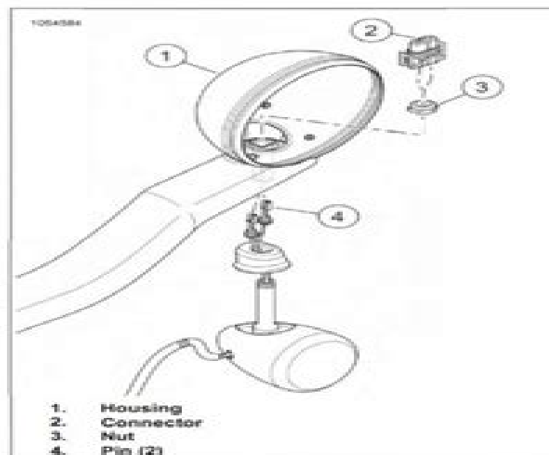
Figure 7-71. Auxiliary Lamp Housing with Incandescent Signal
