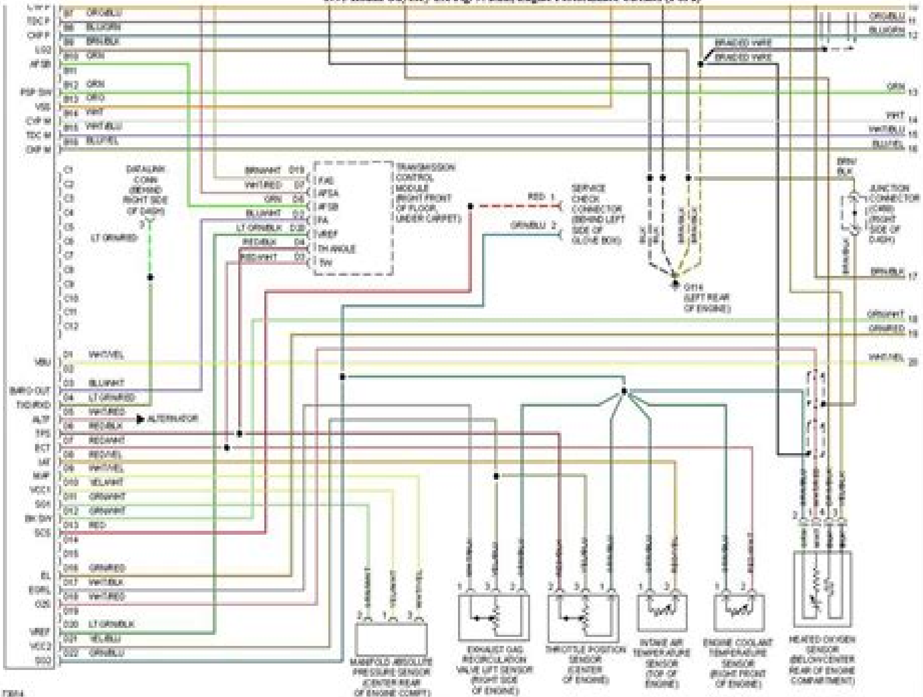
1999 Honda Odyssey EX-V6, Fig. 9-211, Engine Performance Circuits (1 of 3)
