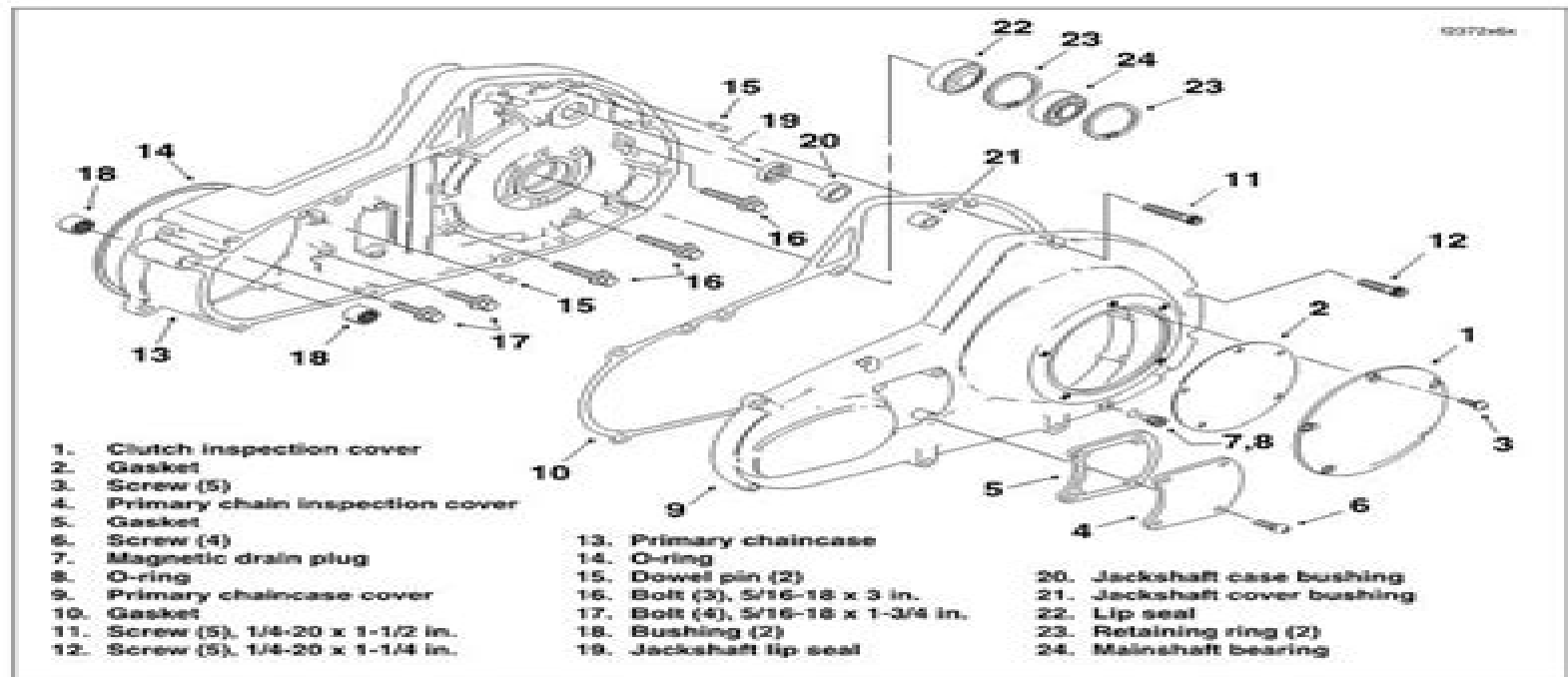
Figure 6-27. Primary Chaincase Assembly
