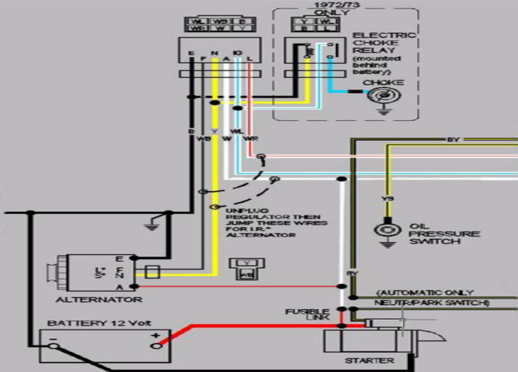
USA wiring spec INTERNALLY REGULATED ALTERNATOR WIRING DIAGRAM DATSUN 510 (1970-72) SEDAN/WAGON
