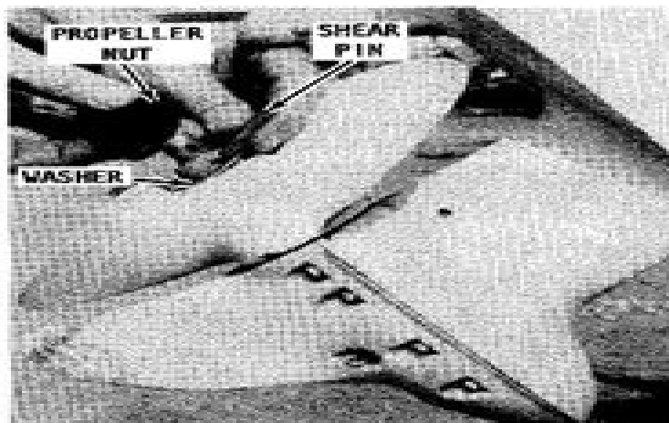
Propeller and associated parts in order, washer, shear pin, and nut, ready for installation.
