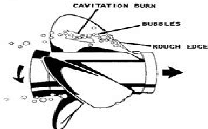
Cavitation (air bubbles) formed at the propeller. Manufacturers are constantly fighting this problem, as explained in the text.
