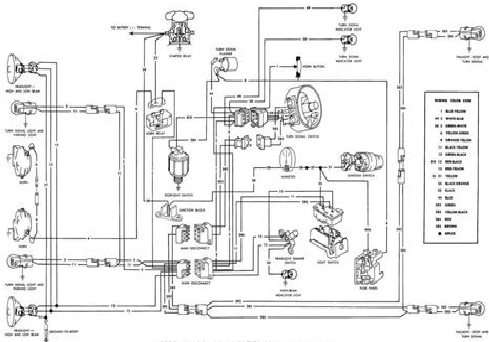
1966 F-100 THRU F-750 SERIES TRUCKS EXTERIOR LIGHTING, TURN SIGNALS AND HORNS
