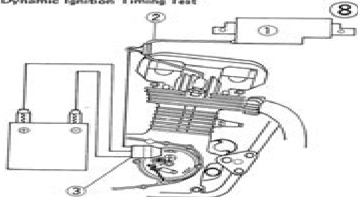
1. Ignition Coil 3. Strobe Light 2. Spark Plug Lead
