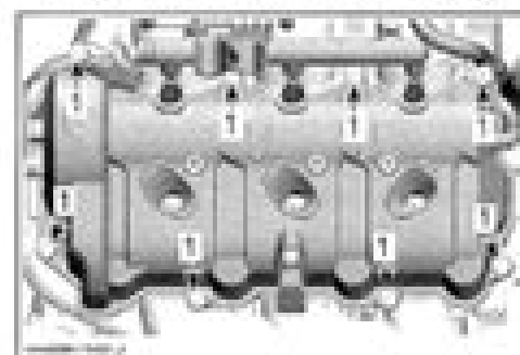
1. Valve cover screws
