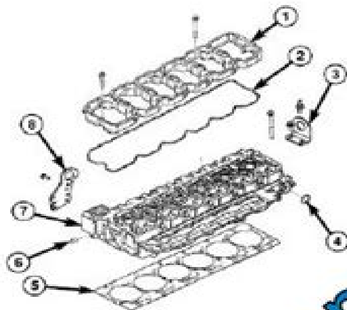
Fig. 70: Cylinder Head Assembly & Timing Cover Courtesy of CHRYSLER GROUP LLC
