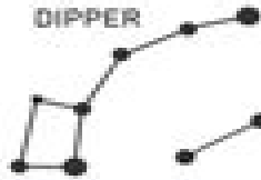
BIG DIPPER
