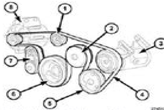
Fig. 2: Drive Belt Tensioners & Accessory Drive Belt Routing Courtesy of CHRYSLER GROUP, LLC
