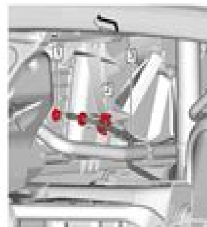
Fig. 154: Transmission Fluid Cooler Inlet and Outlet Pipe @ Radiator Courtesy of GENERAL MOTORS COMPANY
