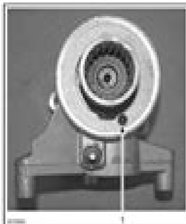
1. Allen screw
