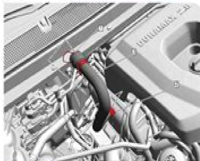
Fig. 27: Blower Inlet Hose
