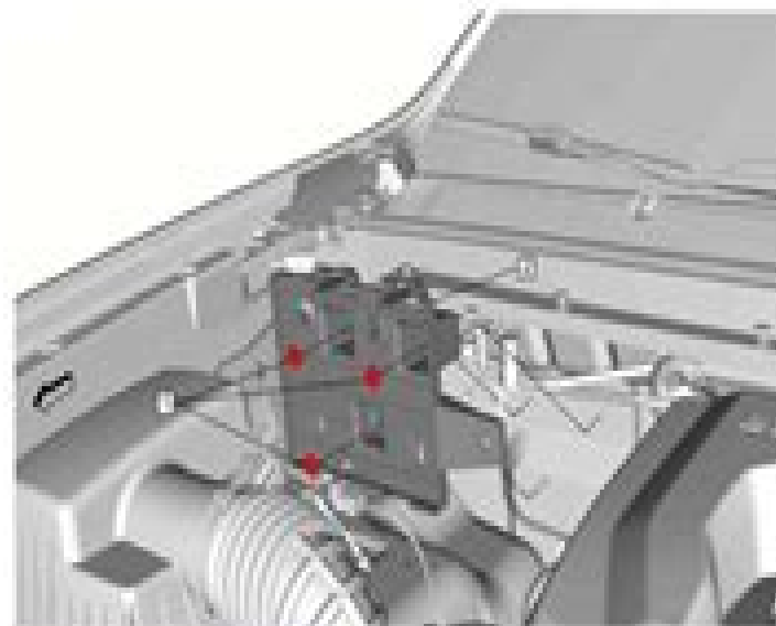
Fig. 26: Engine Control Module Bracket
