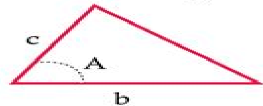
Area with an Angle
