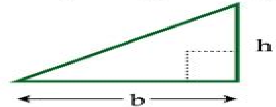
Right Angle Triangle
