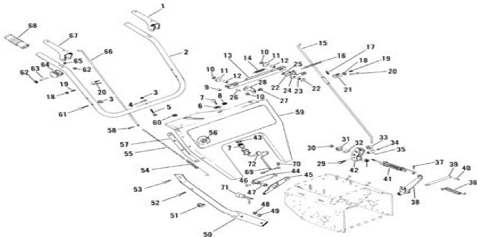
Figure 2-2: Handlebars and Controls
