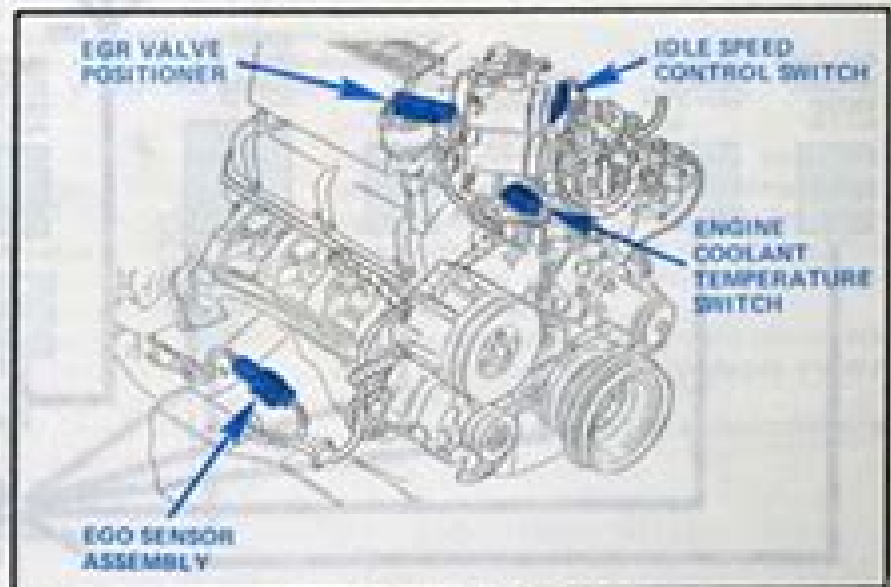
Figure 4 - RH Side of 5.0L EFI Engine
