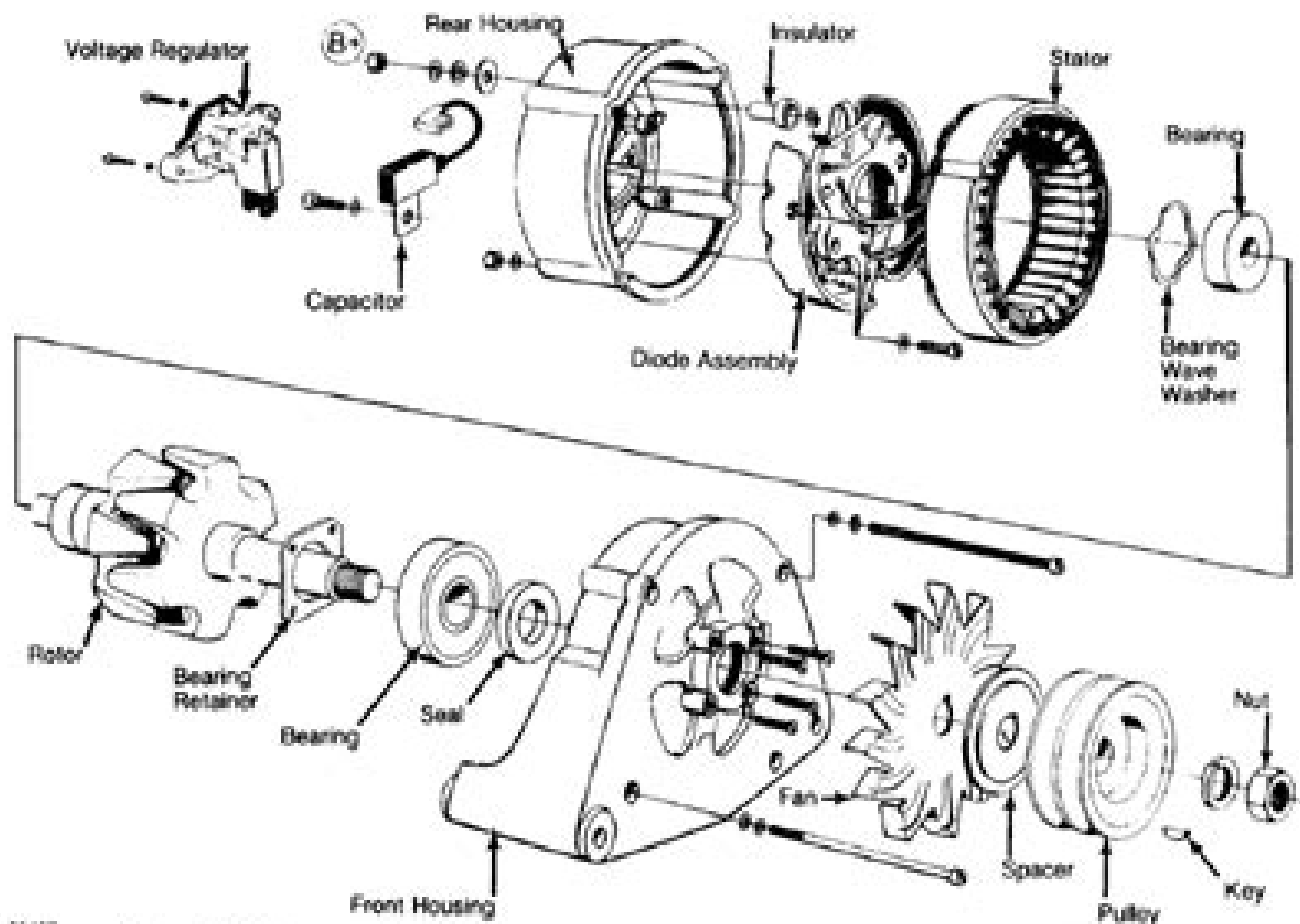
Fig. 2: Exploded View of Bosch 55-Ampere Alternator Courtesy of Mercedes-Benz of North America.
