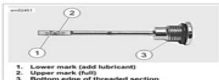
Figure 1-18. Filler Plug/Dipstick
