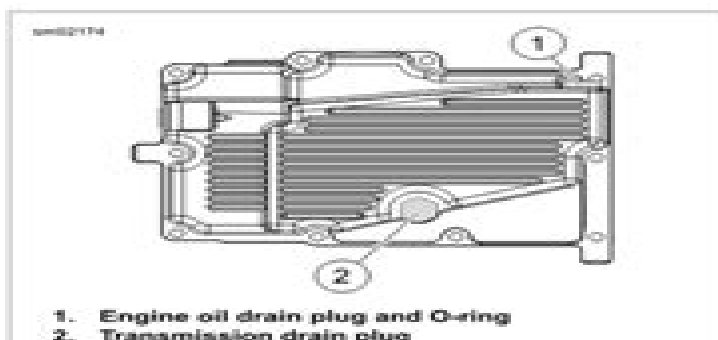
Figure 1-19. Oil Pan
