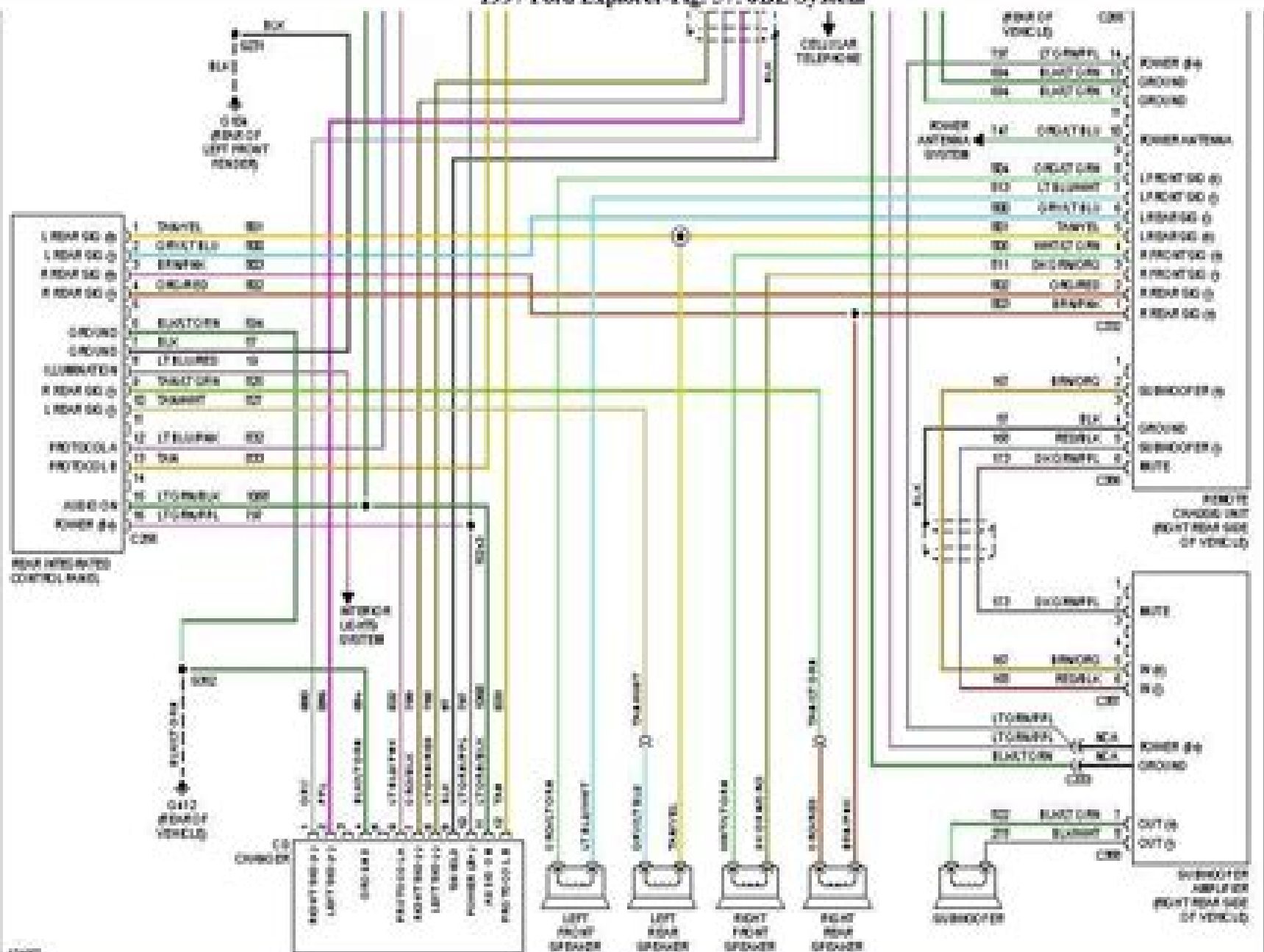
1997 Ford Explorer-Fig. 57: JBL System
