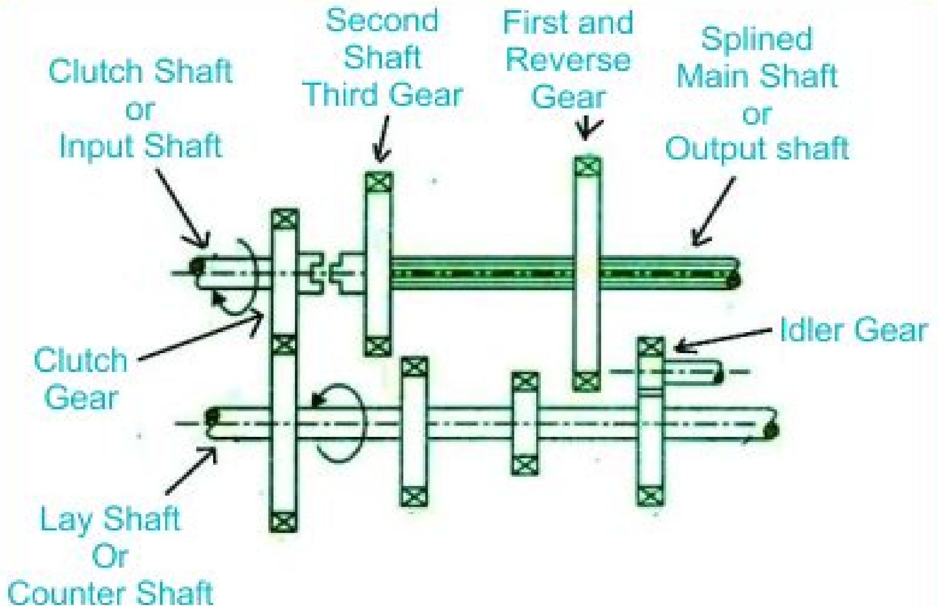
Sliding Mesh Gearboox
