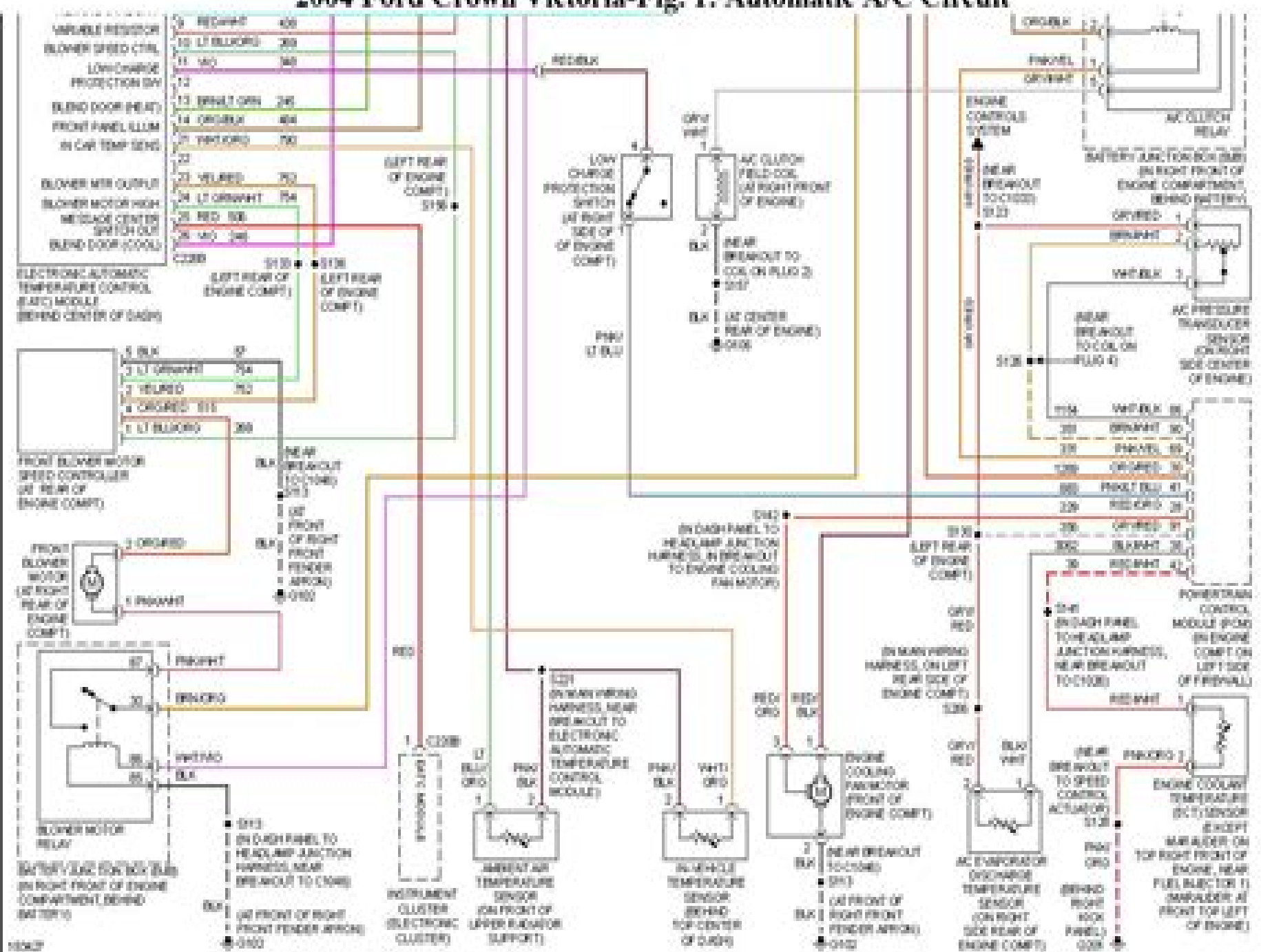
2004 Ford Crown Victoria-Fig. 1: Automatic A/C Circuit
