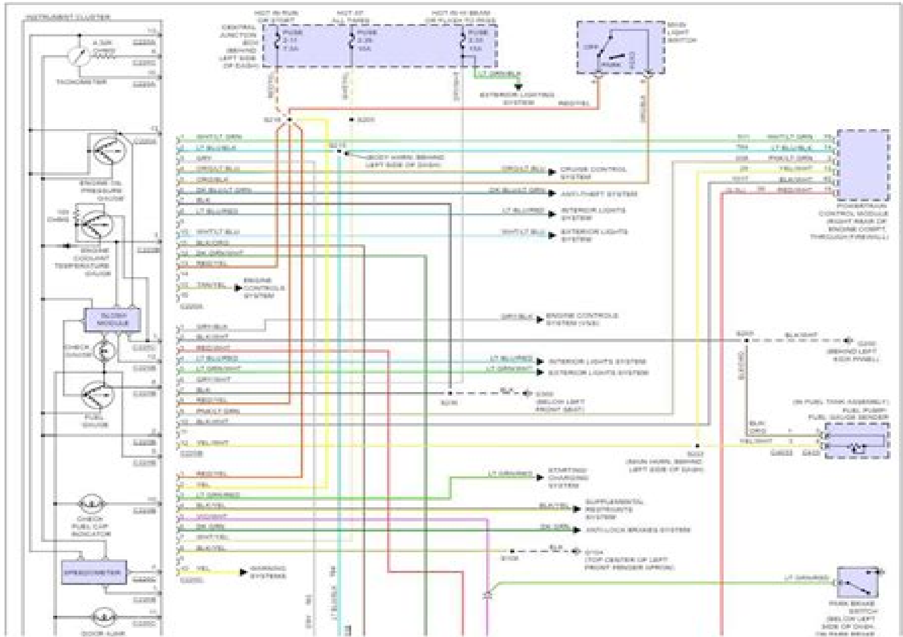
Fig 1: Instrument Cluster Circuit
