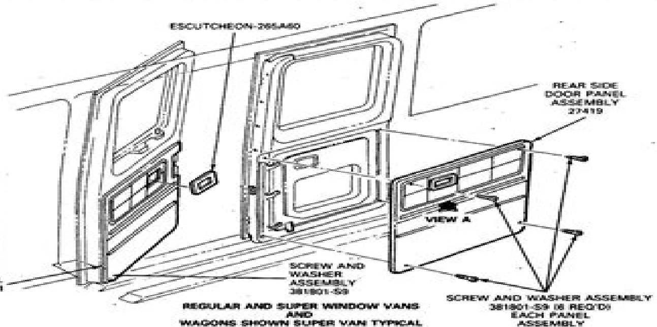
FIG. 8 Side Hinged Door Trim Panel—E-150—E-350
