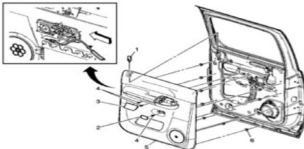
Fig. 6: View Of Rear Side Door Trim Panel (YE9) Courtesy of GENERAL MOTORS CORP.
