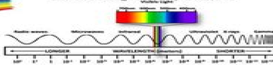
Ultraviolet Light
