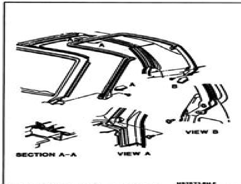
Fig. 8 - Lift-off Panel Opening Weatherstrip Installation
