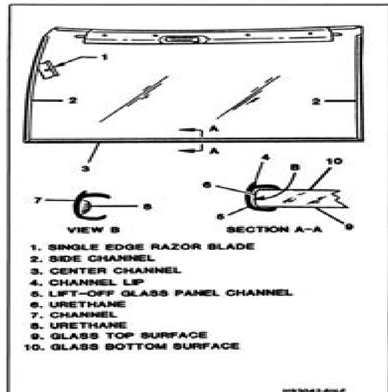
Fig. 9 - Lift-off Glass Panel Channel
