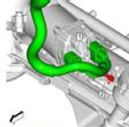
Fig. 24: Steering Gear Electrical Connector And Wiring Harness Clip
